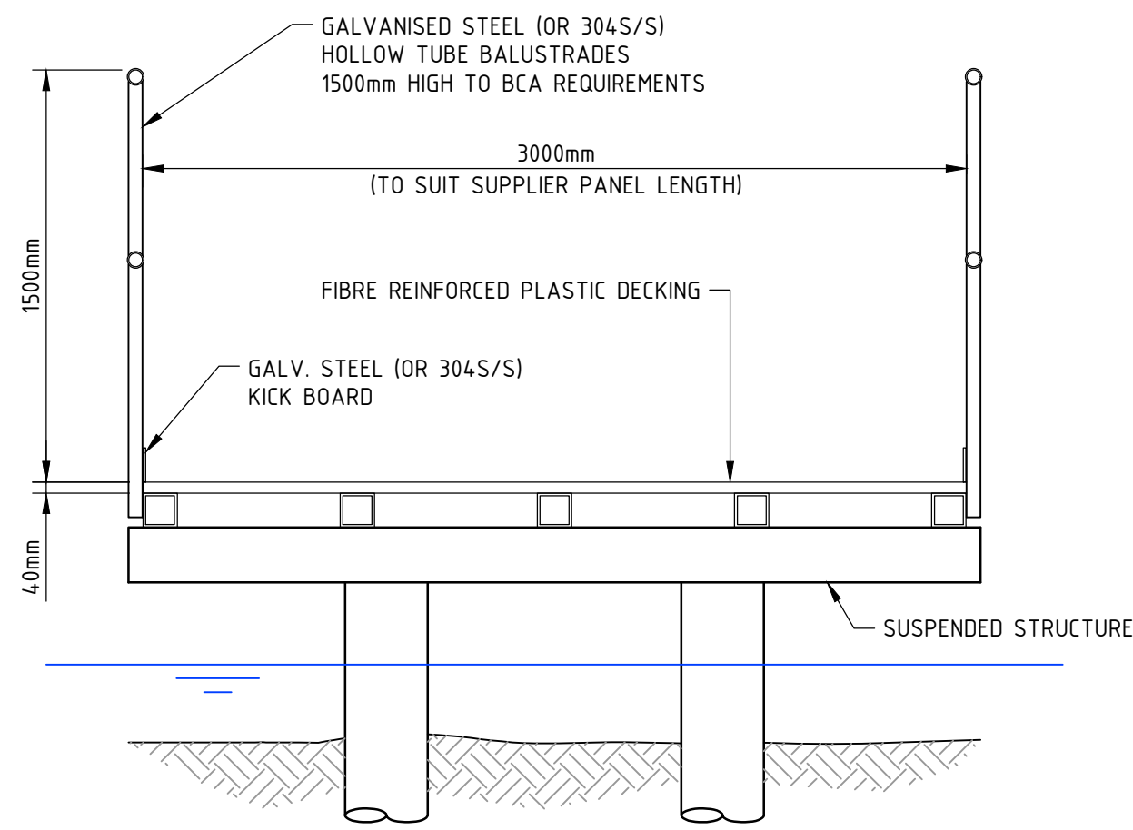
ELEVATED BOARDWALK TYPICAL SECTION (WATER CROSSING) NOT TO SCALE
