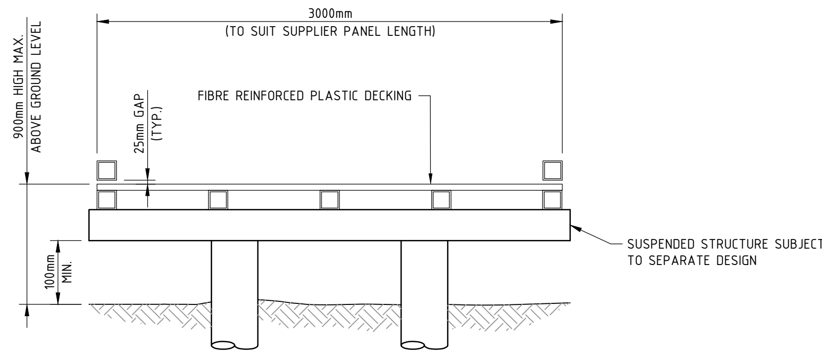
ELEVATED BOARDWALK TYPICAL SECTION (OVERLAND) NOT TO SCALE
