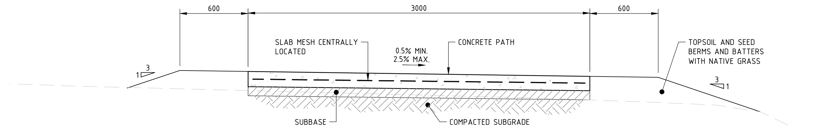
TYPICAL CONCRETE FOOTPATH SECTION (ON GRADE) SCALE 1:20
